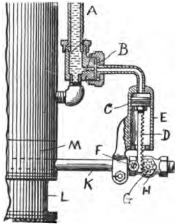
FIG. 254.—Diagram of the Bullard Fuel Cut-off, used on the "Victor" carriage. A is the water level glass; B, the fusible plug; C, the piston to be driven downward by steam when plug is melted; D, rack attached to piston; E, cylinder in which piston slides; F, roller for holding rack in line; G, spur pinion controlling fuel valve; H, fuel valve; K, pipe to burner; L, burner; M, boiler.
